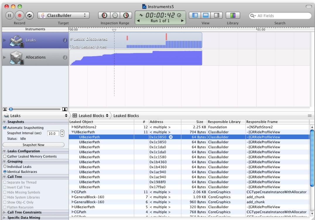
Figure 10.11 Individual leaked memory blocks
