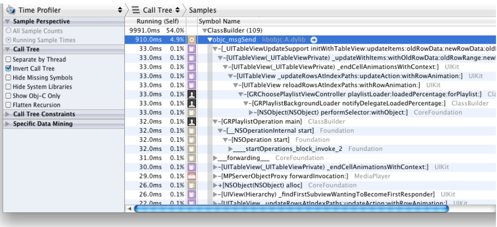
Figure 10.26 Expanding objc_msgSend to see its callers
