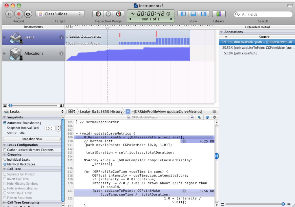
Figure 10.15 Leak with source code
