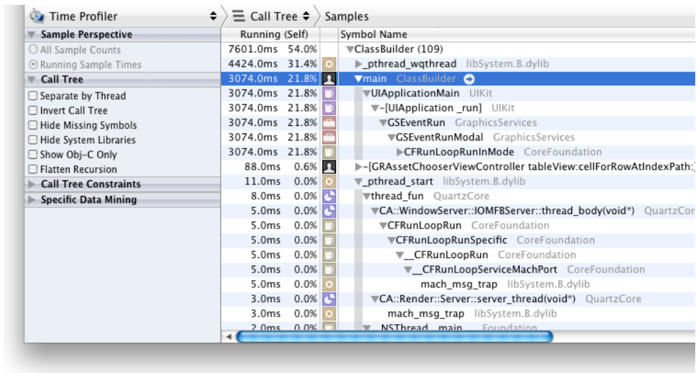
Figure 10.27 Regular call tree
