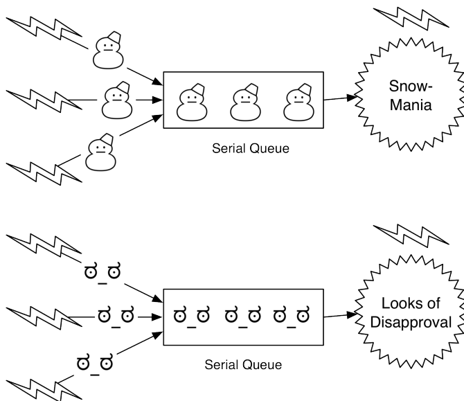
Figure 22.3 Multiple serial queues
