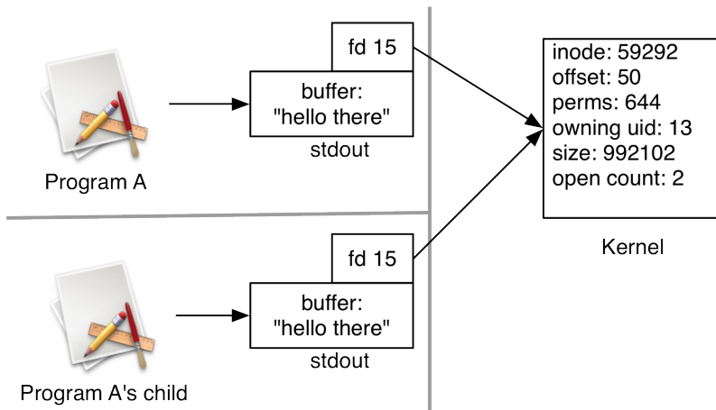
Figure 18.4 Files after fork
