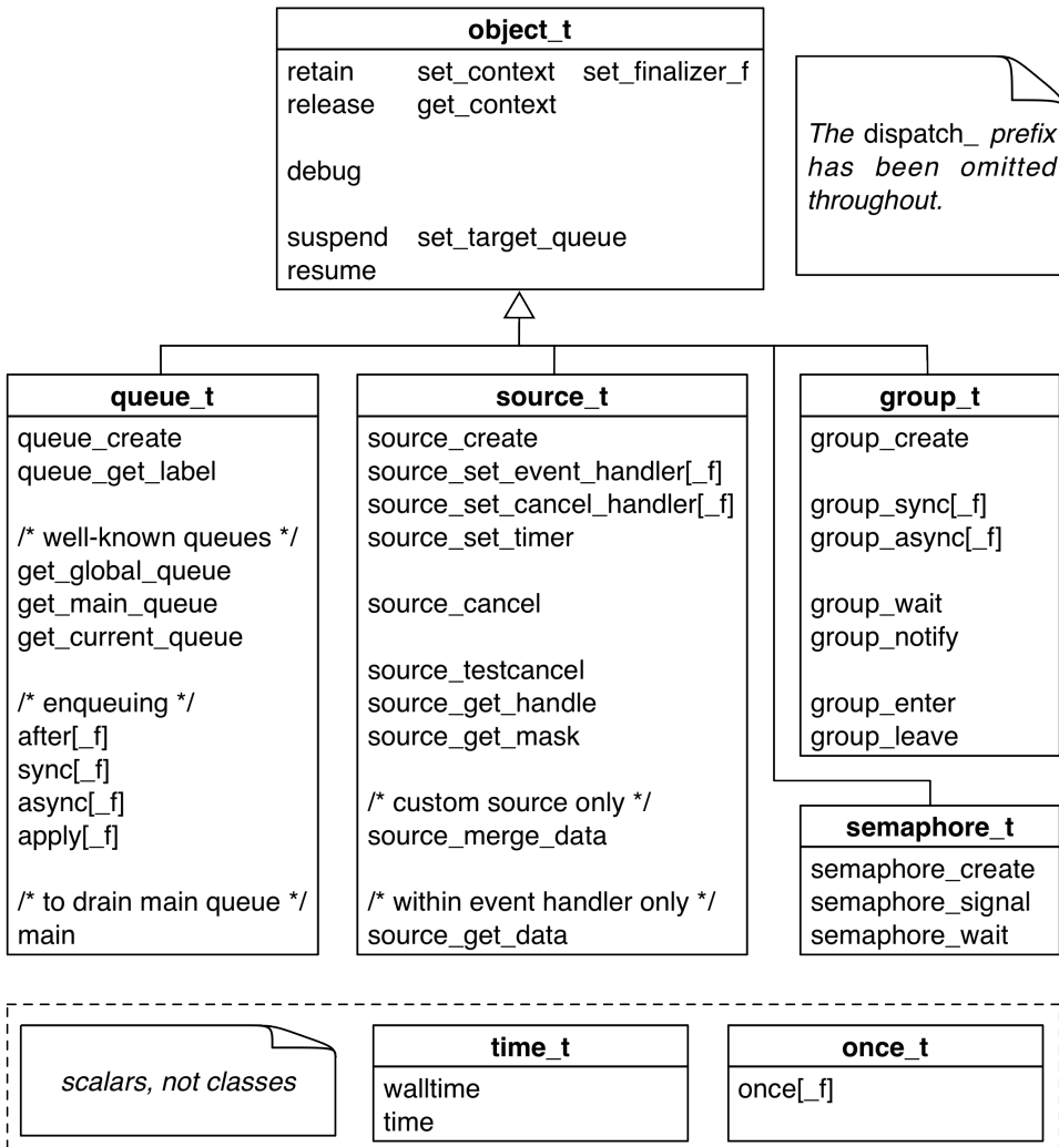
Figure 22.5 Dispatch classes and functions
