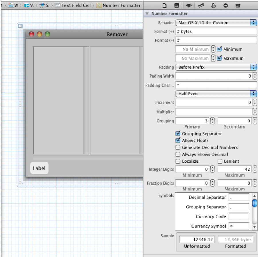
Figure 13.9 Configuring the label's number formatter
