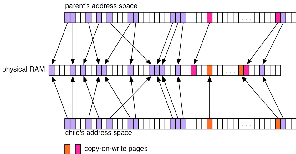
Figure 18.3 Copy on write
