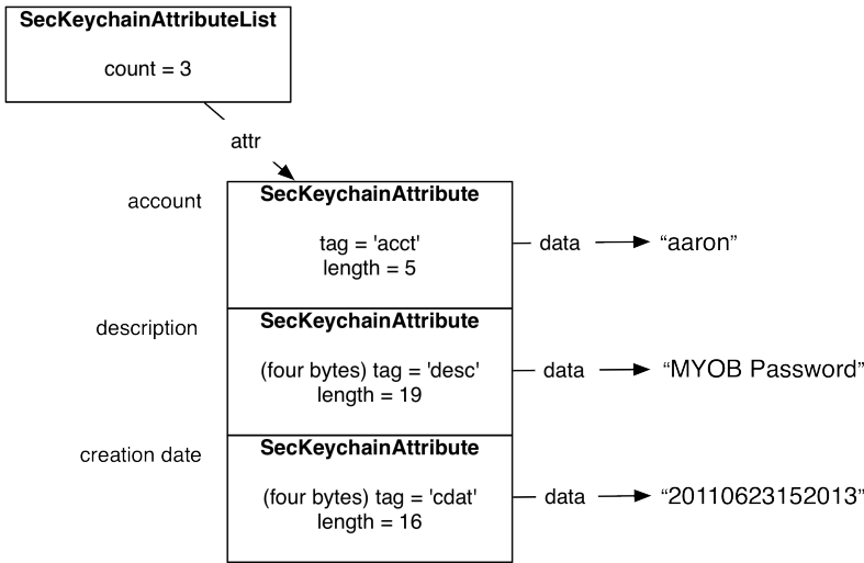
Figure 23.4 Keychain attribute list
