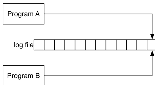
Figure 11.3 Race condition start
