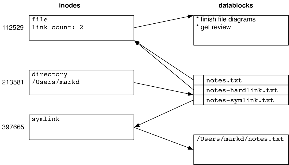
Figure 12.5 Hard and symbolic links
