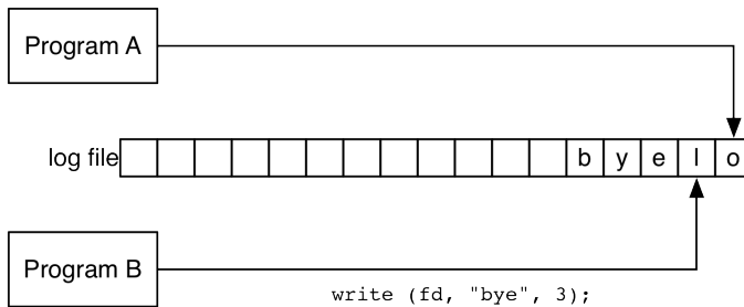
Figure 11.5 Program B clobbers it
