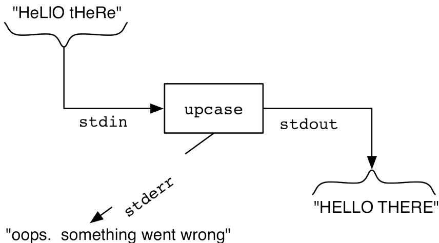
Figure 4.1 The standard file streams
