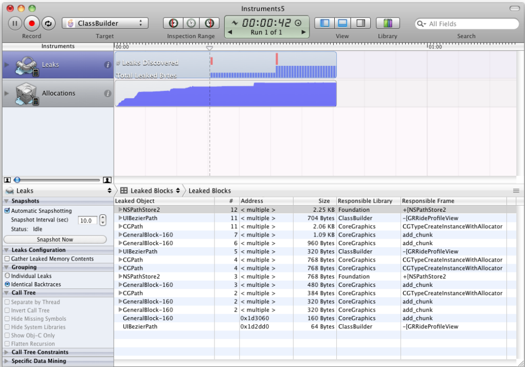
Figure 10.10 Detail panel showing leaked blocks
