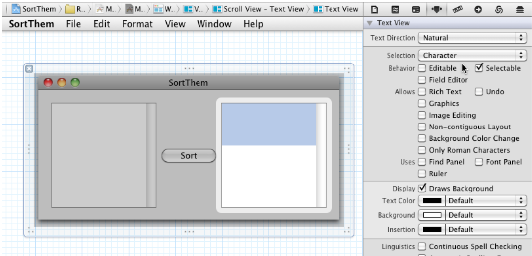
Figure 19.3 Laying out the SortThem window
