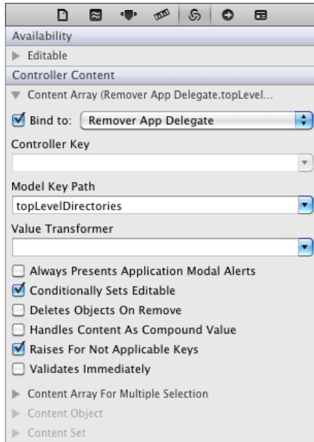
Figure 13.6 Binding the tree controller's contentArray
