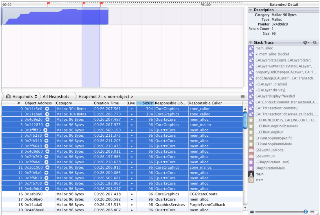
Figure 10.22 Leaking layers stack trace
