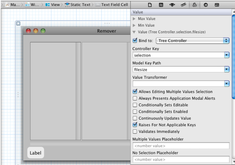
Figure 13.10 Binding the label's contents.
