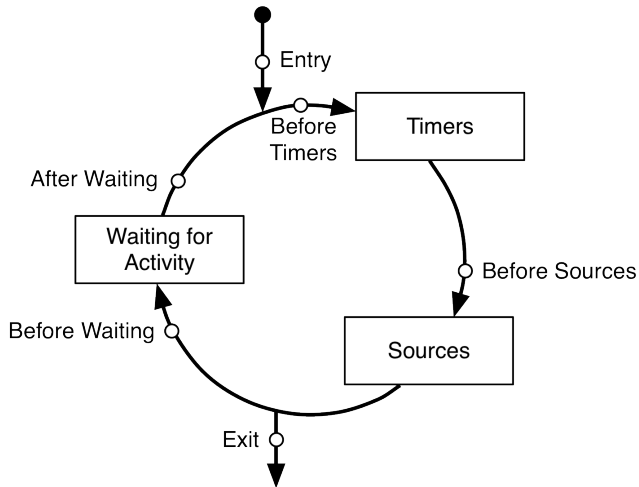
Figure 15.6 Run loop observation points
