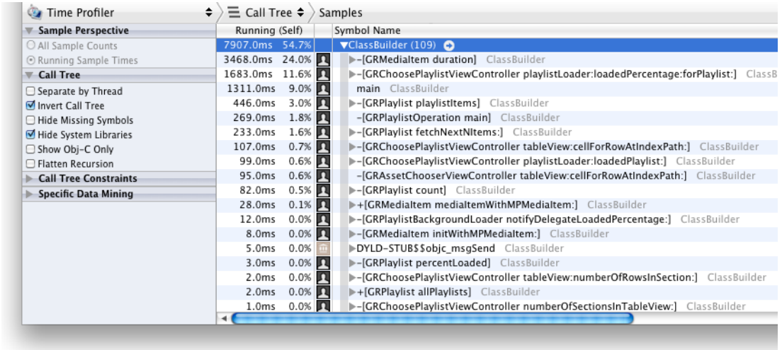
Figure 10.28 Data mining by hiding system libraries
