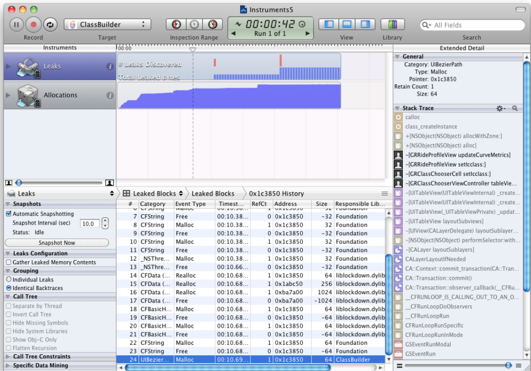
Figure 10.13 Object leak stack trace
