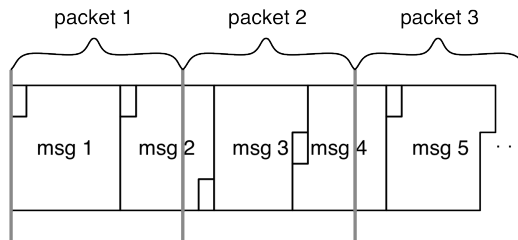
Figure 14.2 Worst-case scenario for messages
