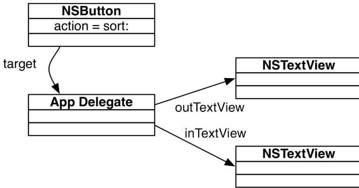
Figure 19.2 SortThem nib file
