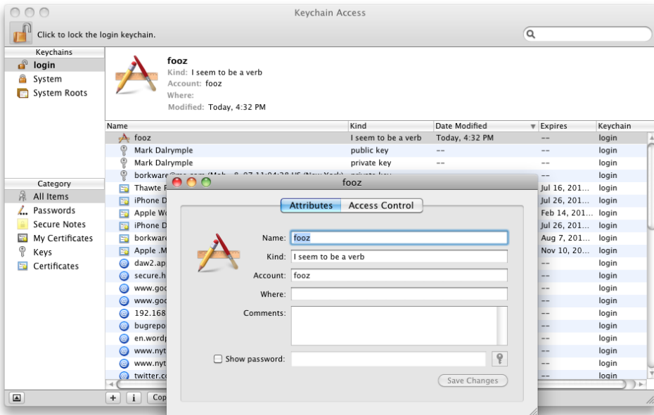
Figure 23.6 Looking at the new keychain item
