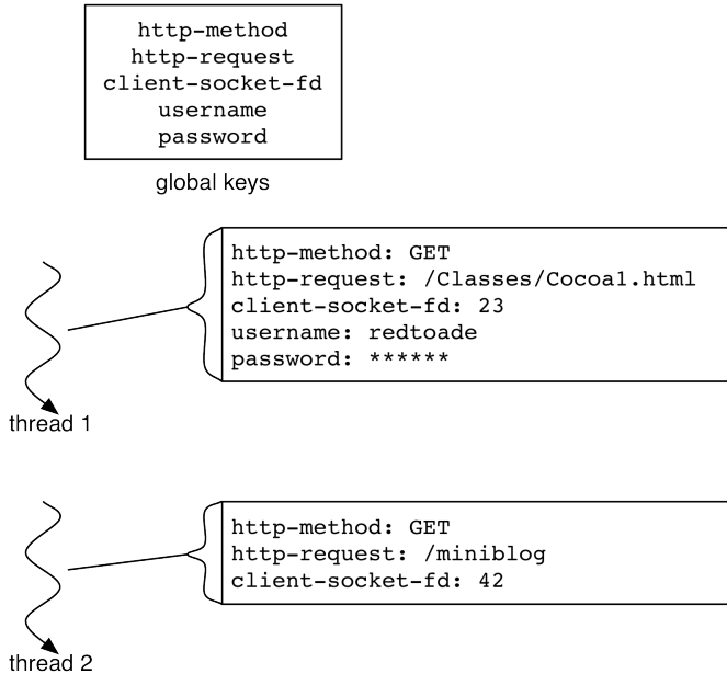
Figure 20.5 Thread local storage
