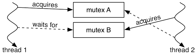
Figure 20.3 Deadlock
