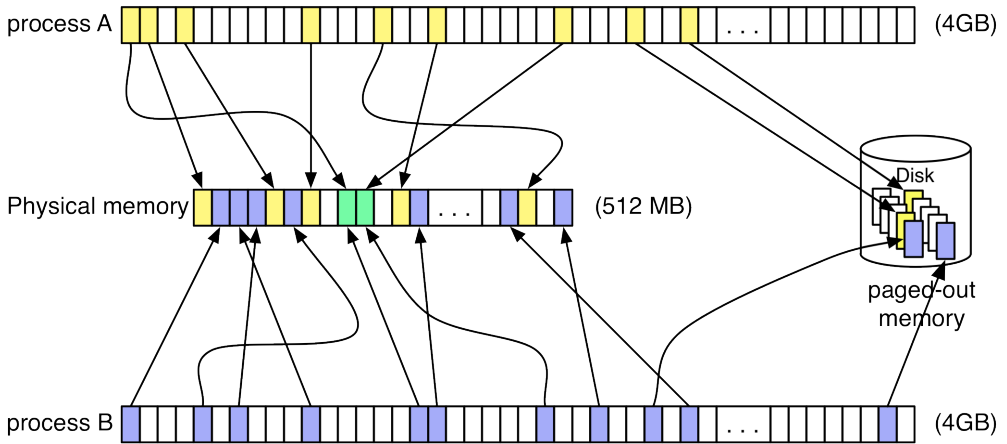
Figure 7.1 Virtual memory
