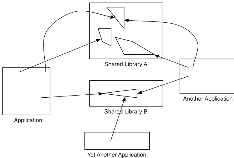
Figure 6.3 Shared libraries
