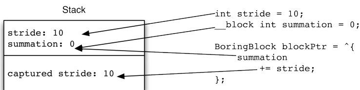
Figure 3.1 Block storage starts on the stack
