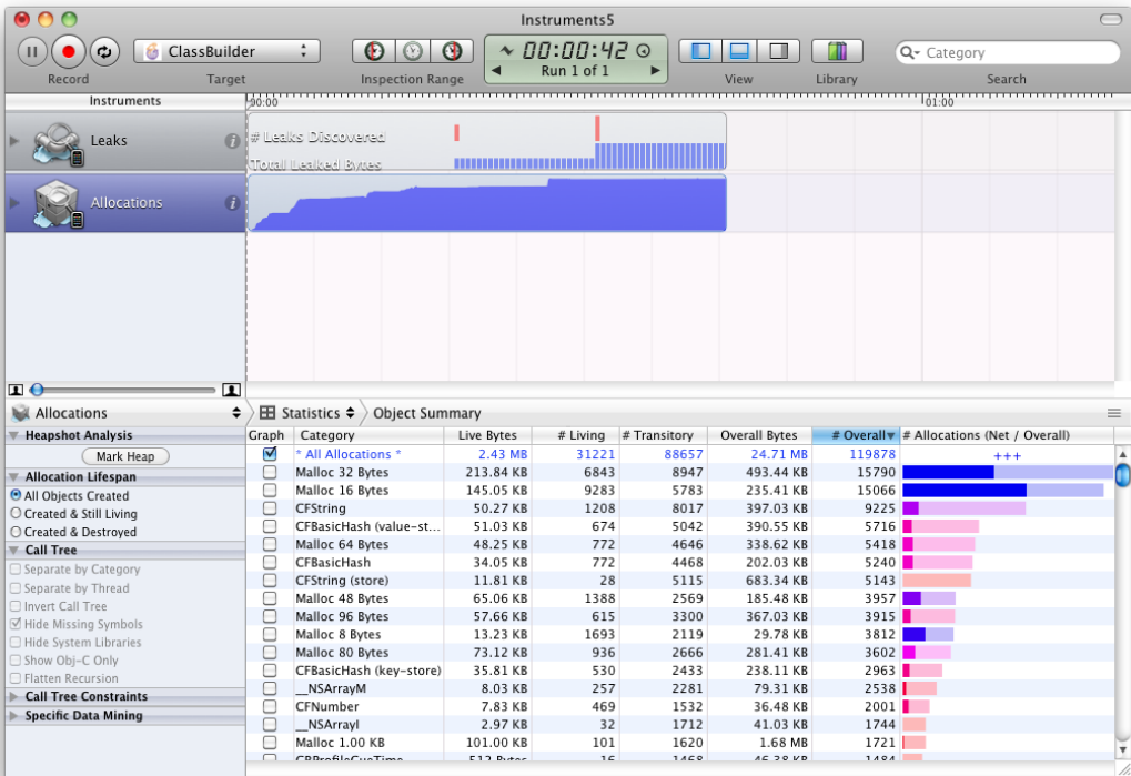
Figure 10.8 Instruments window after running the application
