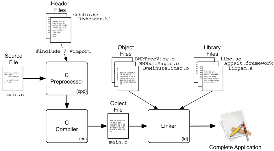
Figure 1.1 The compiler pipeline
