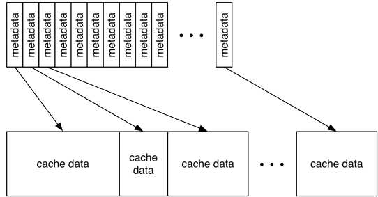
Figure 10.4 Good locality of reference
