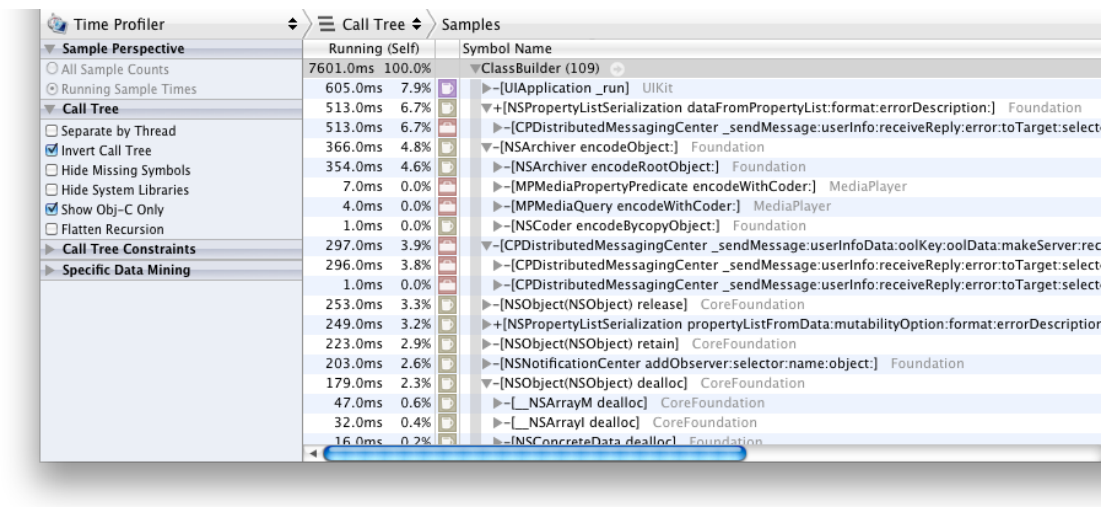
Figure 10.29 Data mining by showing Objective-C only
