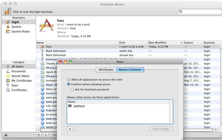
Figure 23.7 Keychain item default access
