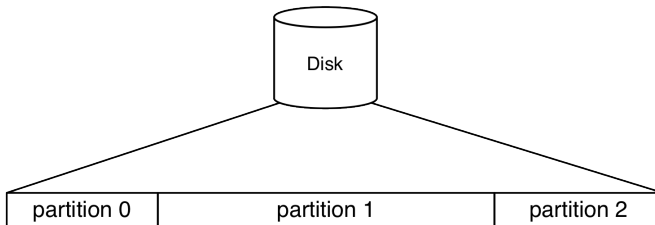
Figure 12.1 Partitions
