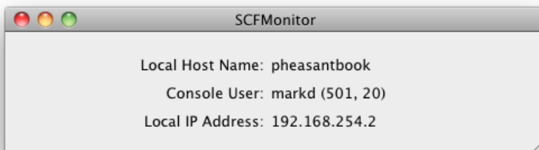
Figure 15.3 SCFMonitor window
