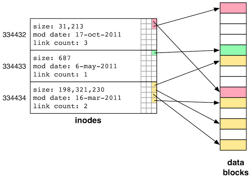
Figure 12.3 inodes
