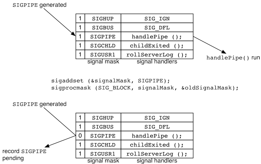
Figure 5.1 Blocking signals
