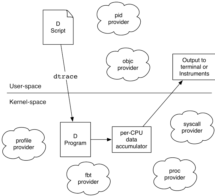
Figure 9.2 DTrace workflow
