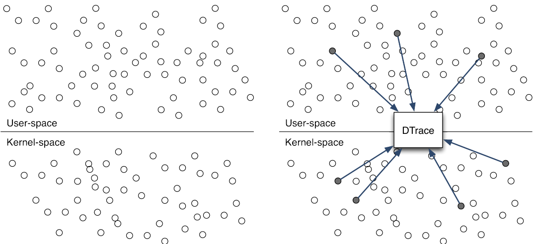
Figure 9.1 DTrace probes
