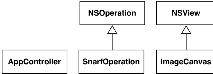
Figure 21.5 ImageSnarfer classes
