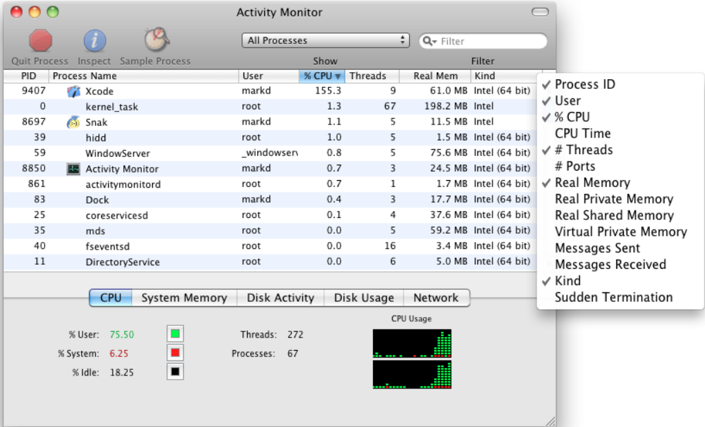
Figure 10.6 Activity Monitor
