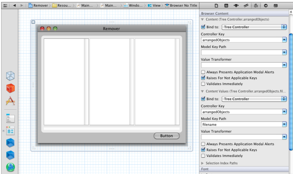
Figure 13.7 Binding the browser's arrangedObjects
