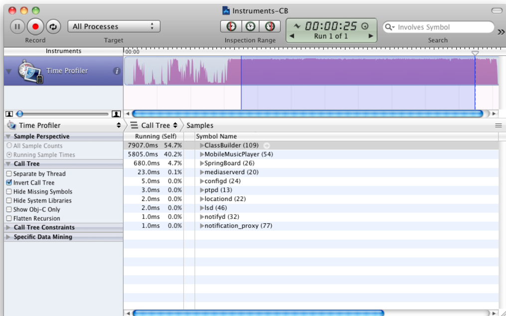
Figure 10.24 Time Profiler instrument sample run
