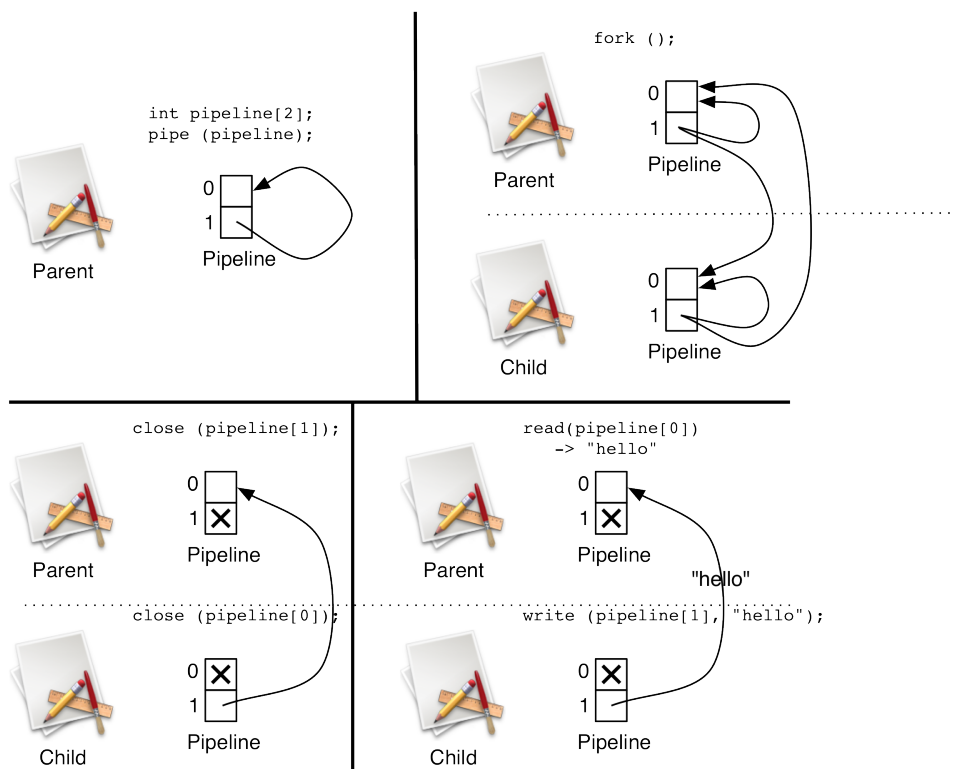
Figure 18.5 Pipe and fork
