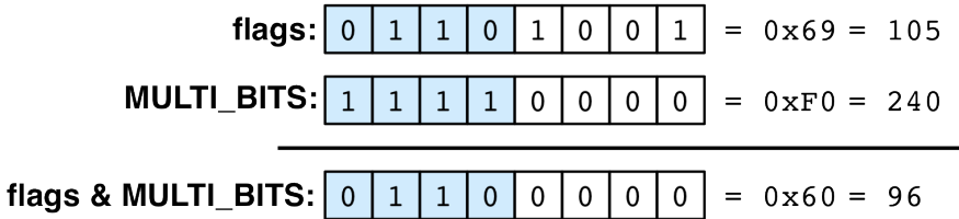
Figure 1.13
