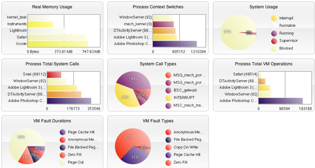
Figure 10.35 Highlight views
