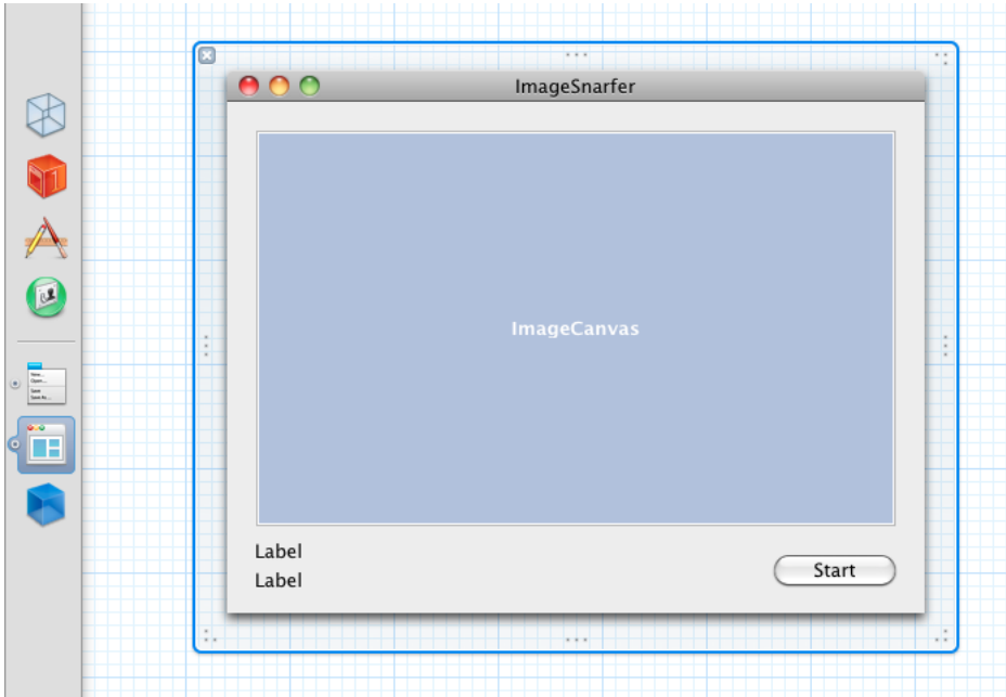
Figure 21.6 ImageSnarfer window
