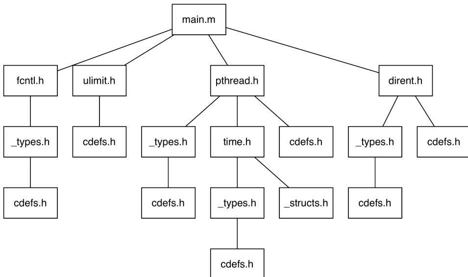
Figure 1.2 Nested #includes
