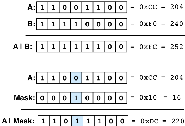
Figure 1.6 Bitwise OR
