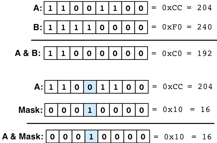
Figure 1.5 Bitwise AND
