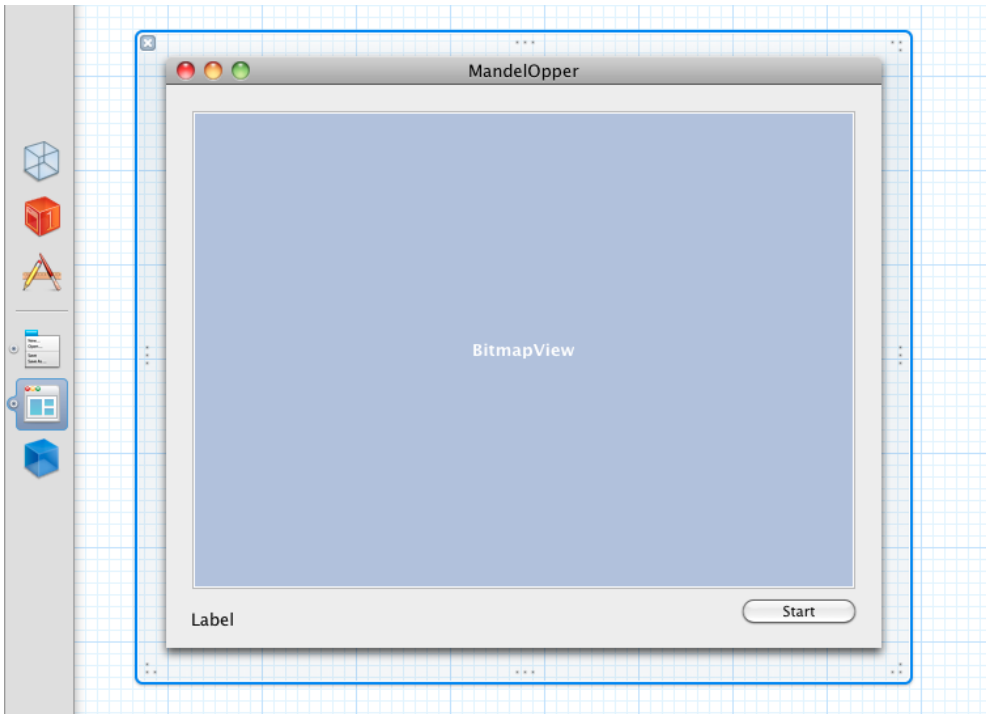
Figure 21.3 MandelOpper window
