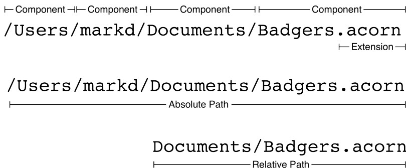
Figure 13.1 Path components
