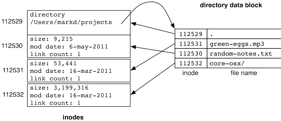
Figure 12.4 Directory structure
