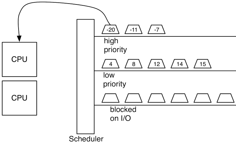
Figure 18.1 The scheduler
