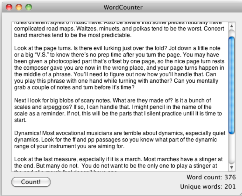
Figure 22.6 WordCounter screenshot
