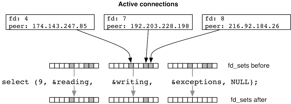
Figure 14.1 select()
