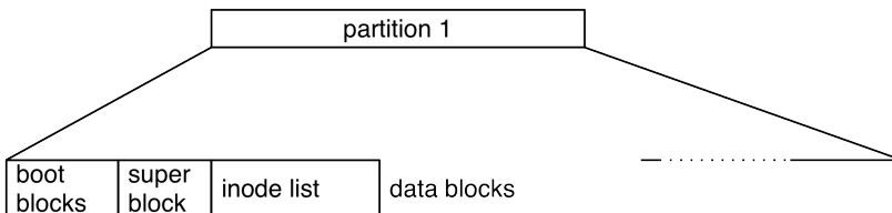
Figure 12.2 Filesystem
