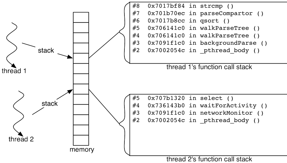
Figure 20.1 Thread stacks
