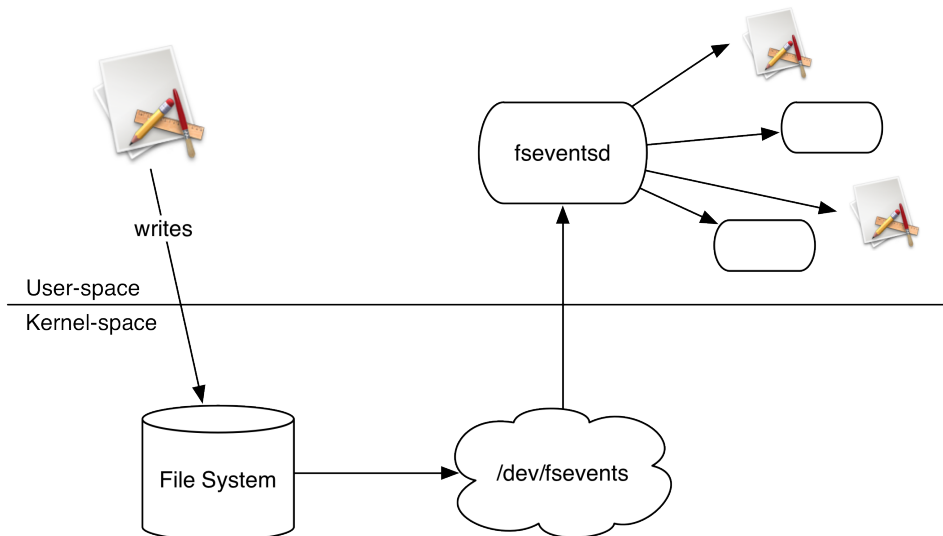
Figure 16.3 fseventsd notifying a file system change
