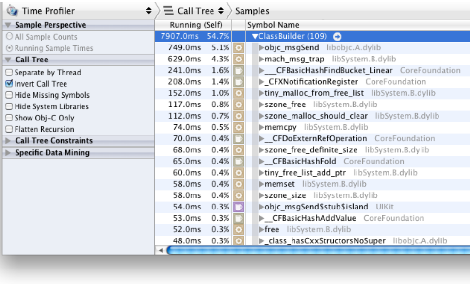
Figure 10.25 Time Profiler call tree
