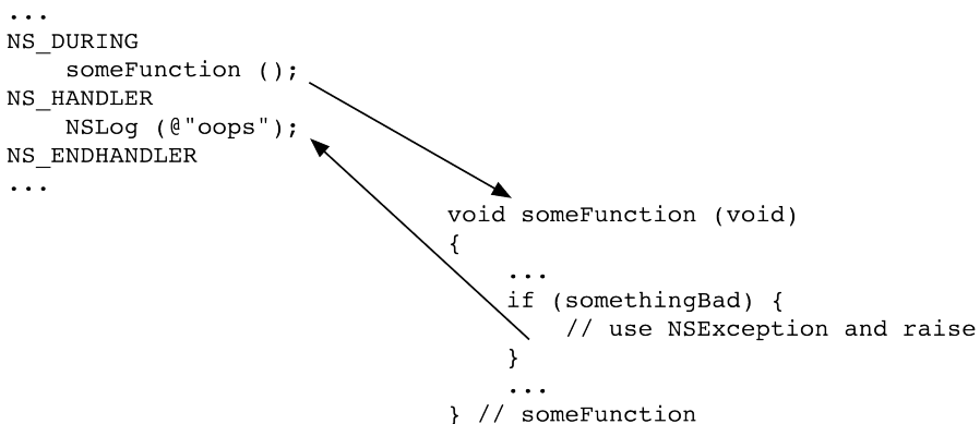
Figure 5.2 Exception flow of control
