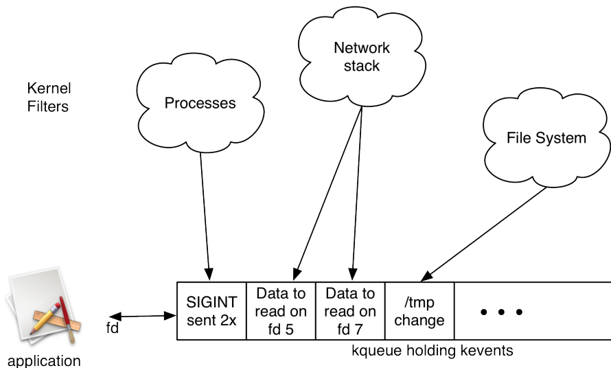
Figure 16.1 Kernel filters adding new events to a kqueue
