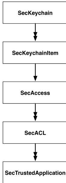
Figure 23.5 Keychain data structures
