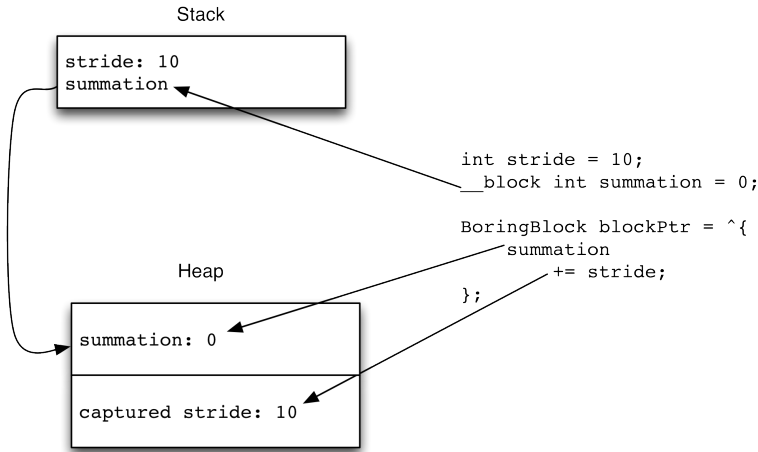
Figure 3.2 Copies get moved to the heap
