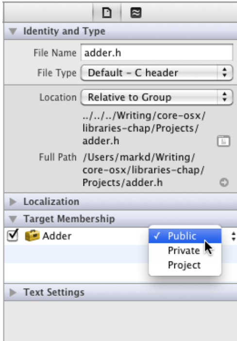
Figure 6.6 Setting the header's public target membership
