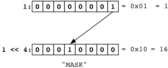
Figure 1.9 Bitwise shift
