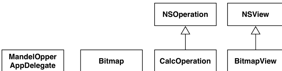
Figure 21.2 MandelOpper classes
