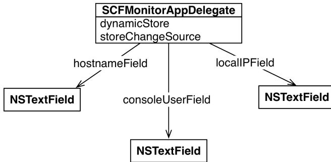
Figure 15.5 SCFMonitor object diagram
