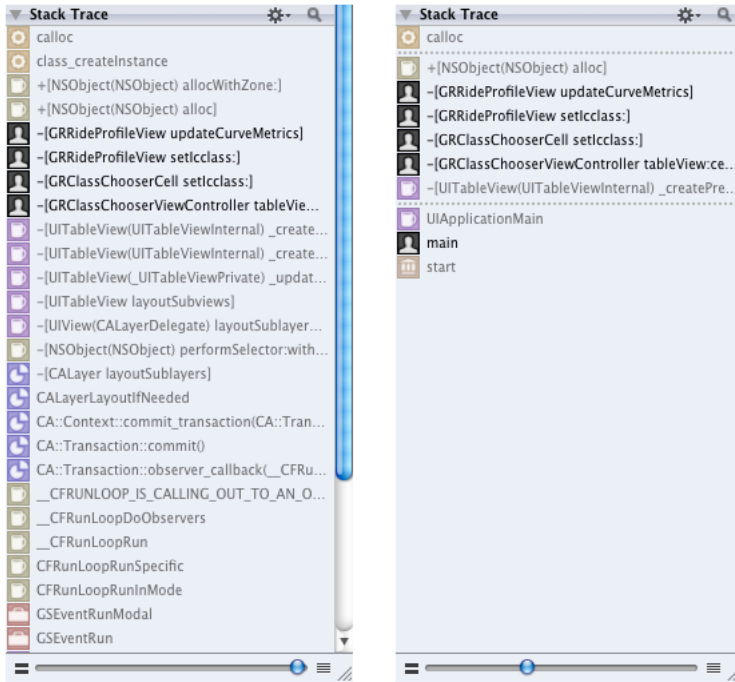
Figure 10.14 Full and reduced stack traces
