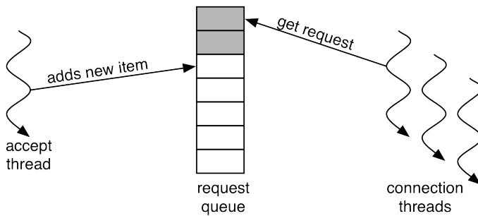
Figure 20.4 Server request queue
