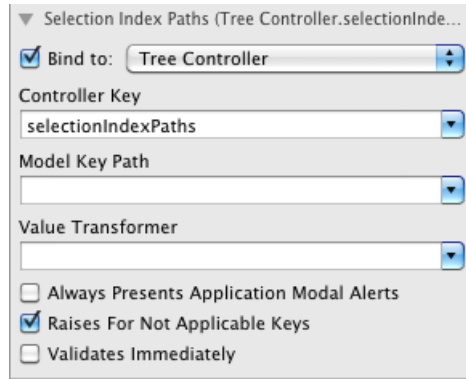
Figure 13.8 Binding the browser's selection index paths
