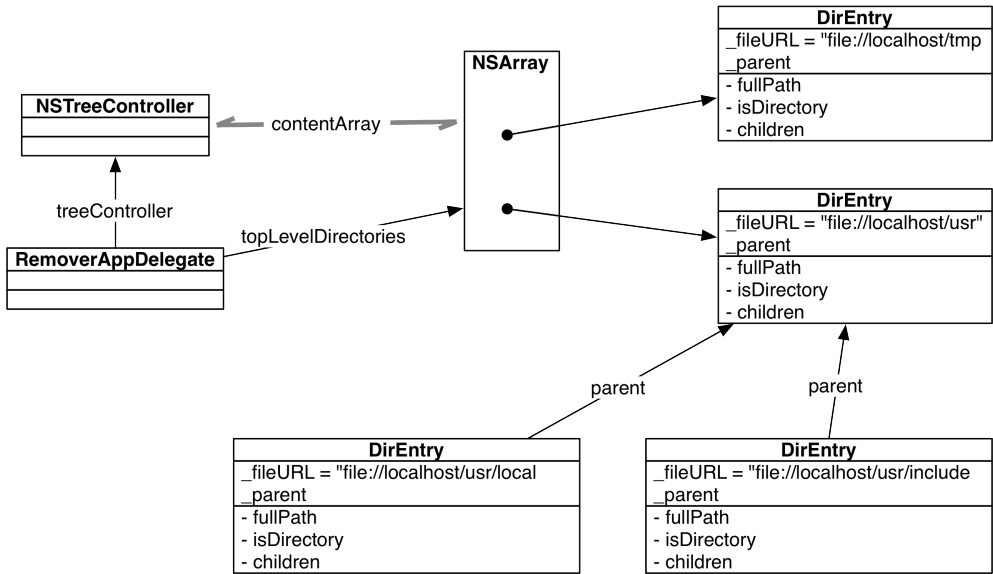
Figure 13.4 Class diagram for Remove app
