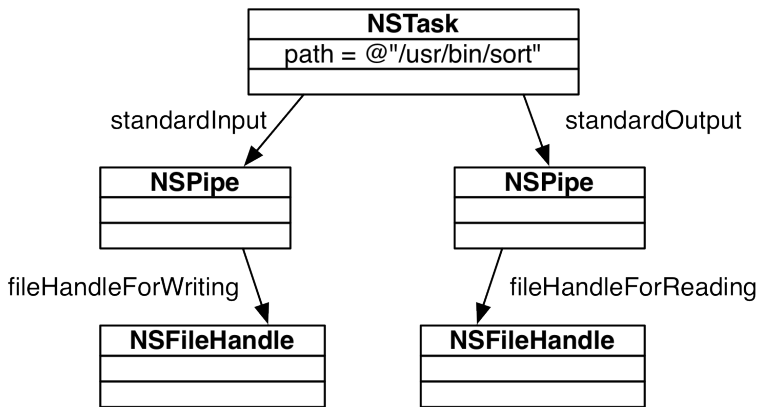
Figure 19.4 SortThem object diagram
