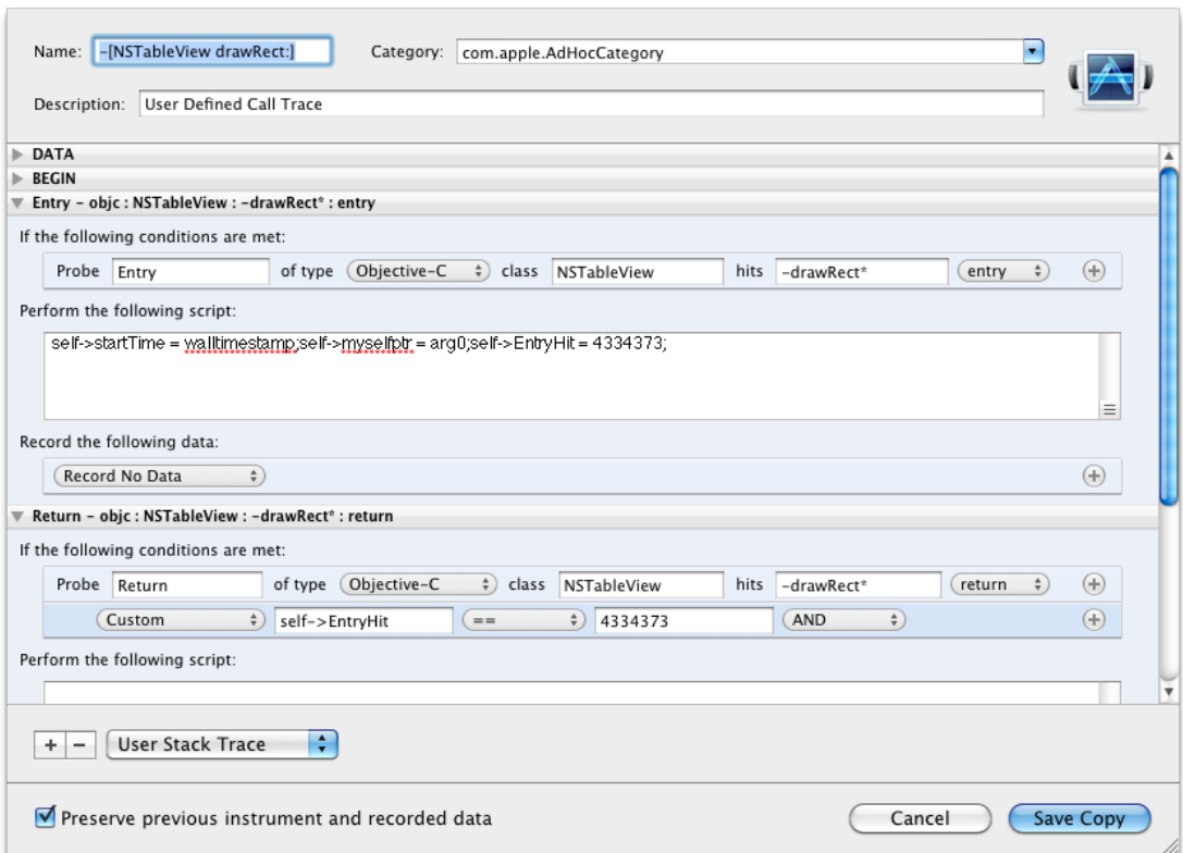
Figure 10.37 DTrace instrument configuration
