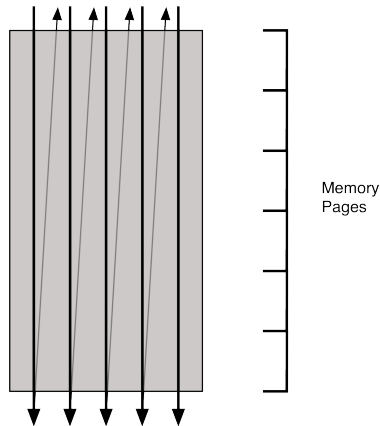
Figure 10.2 Bad memory access pattern
