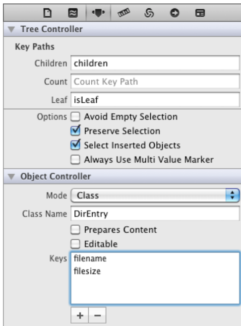
Figure 13.5 Configuring the tree controller's bindings
