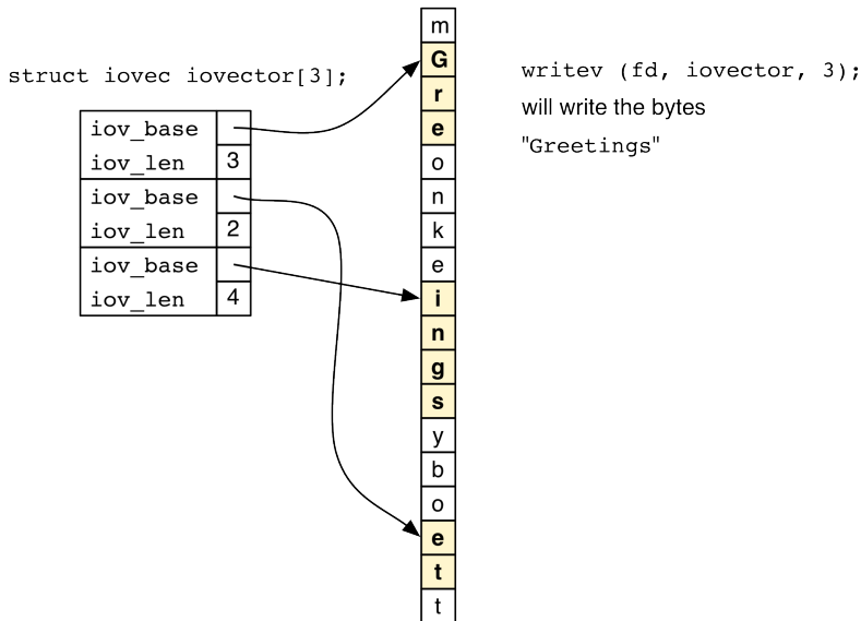
Figure 11.6 Scatter / Gather I/O
