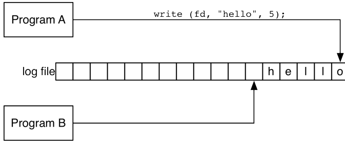
Figure 11.4 Program A writes its data
