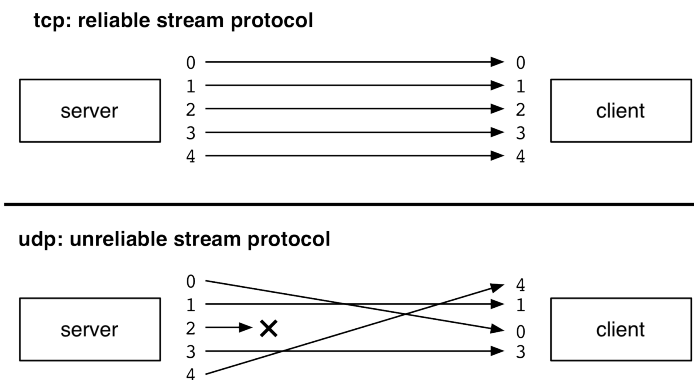
Figure 14.3 TCP versus UDP
