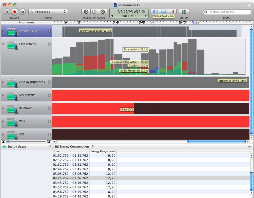
Figure 10.30 The Power-oriented instruments
