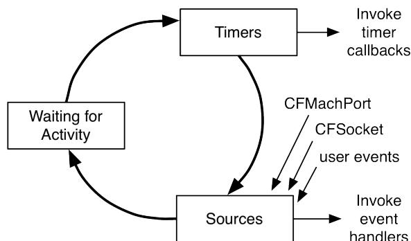
Figure 15.1 The run loop
