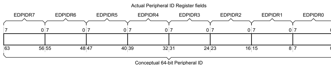
Figure K2-3 Mapping between Peripheral ID Registers and a 64-bit Peripheral ID Value
