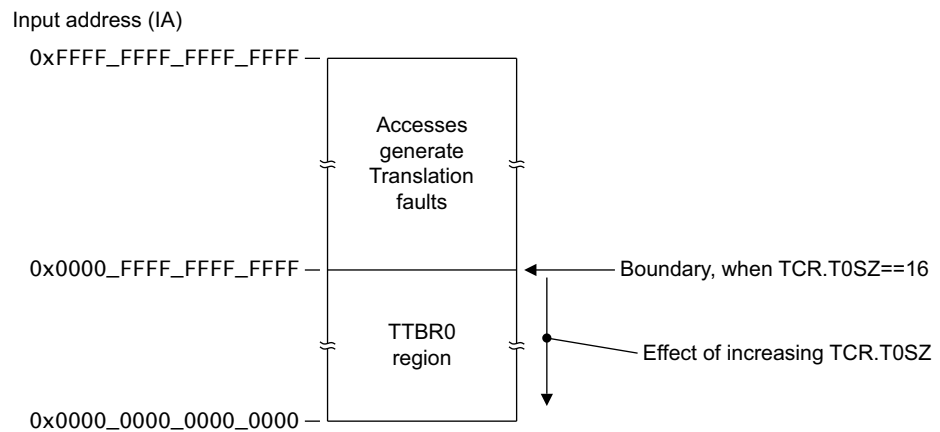
Figure D4-2 AArch64 input address map when using a single TTBR
