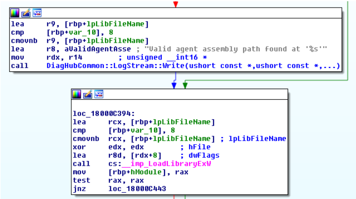
Figure 5: AddAgent Function
