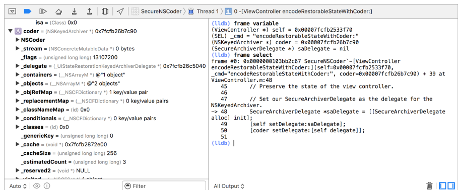
Figure 5-3: Examining frame variables from the command line and the GUI
