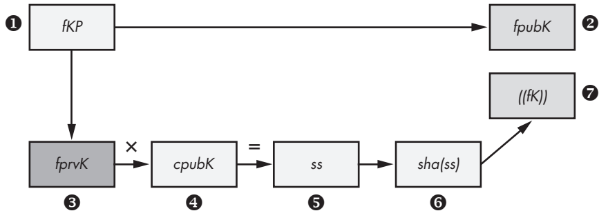
Figure 13-3: Key generation and wrapping. Note that the file private key ③ is transient and is discarded after the wrapped file key is stored in the file metadata.
